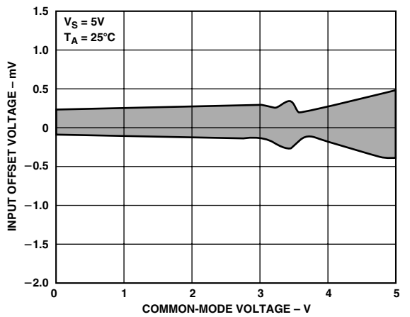
TPC 6. Input Offset Voltage vs. Common-Mode Voltage
